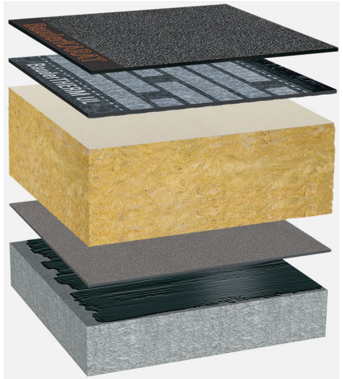
Sustav: BG_MIFA-P_K_01
